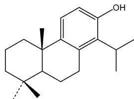
FIGURE 1: Structure of totarol (14-isopropyl-8,11,13-podocarpatrien-13-ol).
